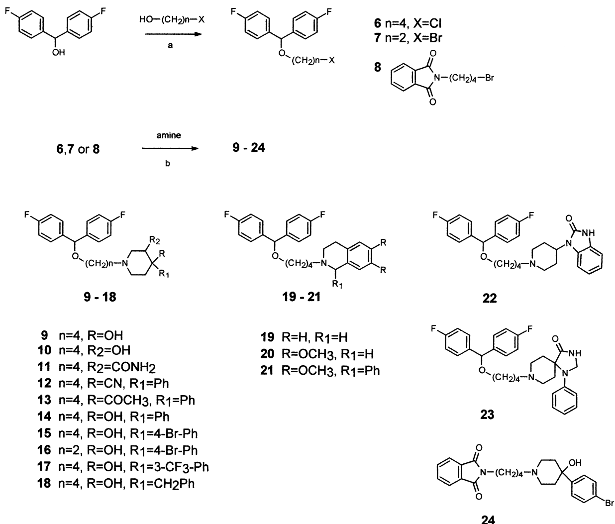
Scheme 1. (a) concd \text{H}_2\text{SO}_4 , \text{PhCH}_3 ; (b) \text{K}_2\text{CO}_3 , KI, DMF, 60–70 °C.
